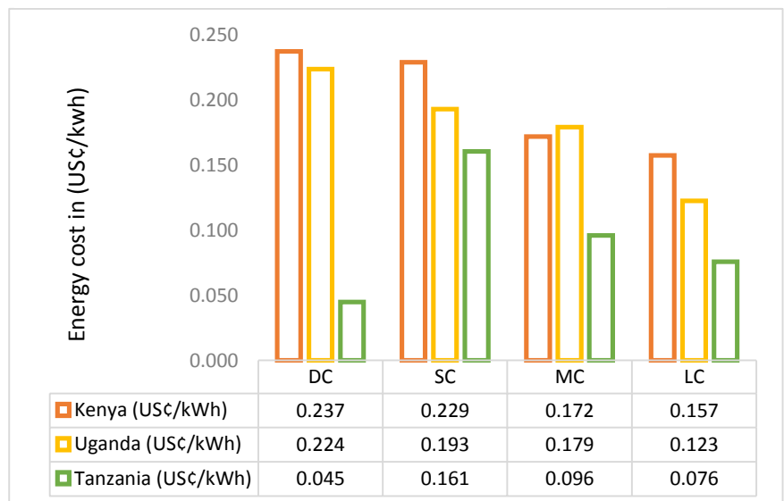
Figure 5: Average electricity prices (US$/kWh) over the 9 month period
